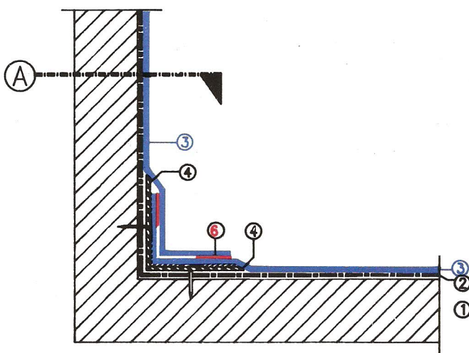
CORNER DETAIL
